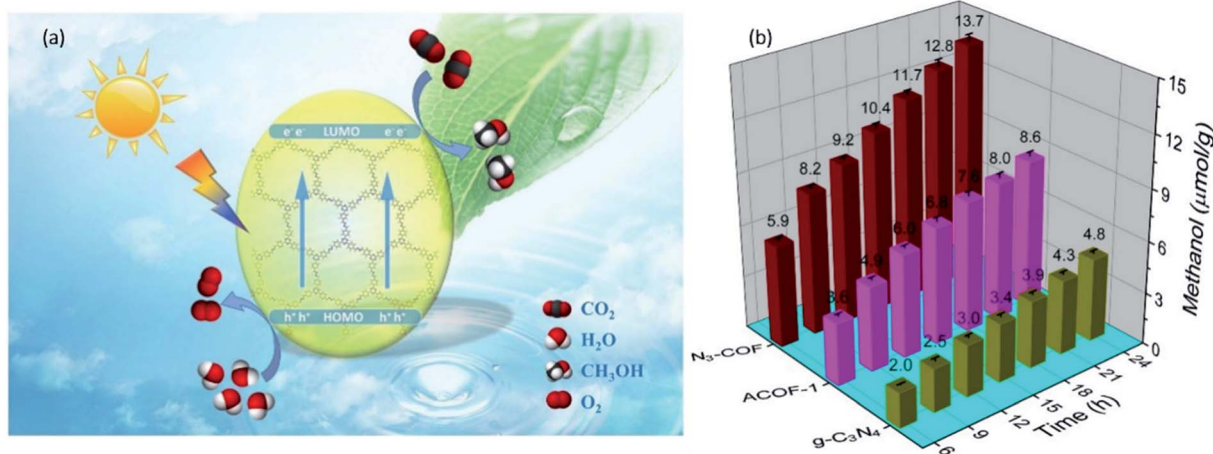
Fig. 11 (a) Schematic illustration for the photocatalytic reduction of CO_2 to CH_3OH over azine-based COFs. (b) Comparison of the amount of CH_3OH produced using ACOF-1, N_3 -COF and g-C_3N_4 as the photocatalysts. Adapted with permission from ref. 88. Copyright 2018, Elsevier B.V.
