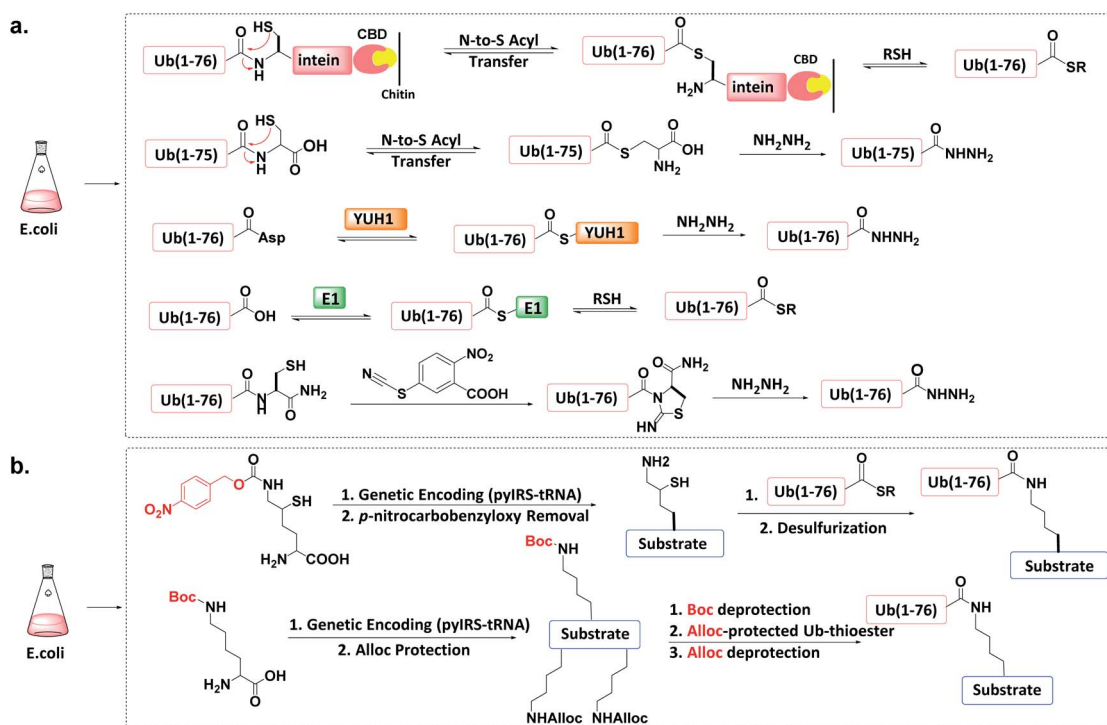
Fig. 6 Protein semi-synthesis of Ub conjugate. (a) Recombinant production of Ub thioesters. (b) Recombinant introduction of isopeptide bonds.
