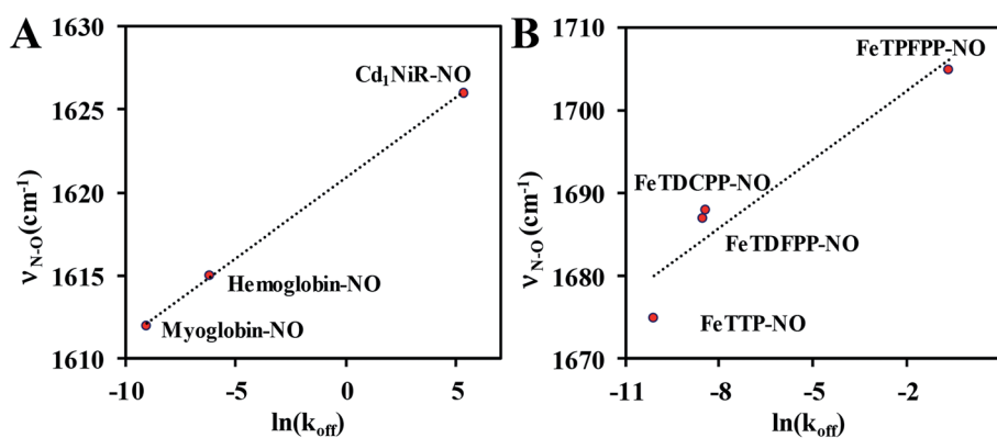
Fig. 2 Correlation between N–O stretching frequency 16–18 and rate of NO dissociation: 19–21 (A) in six-coordinate heme nitrosyls in enzyme systems; (B) in synthetic Fe-porphyrin nitrosyl complexes, TTP ( p -tolyl), TDFPP (2,6-difluorophenyl), TDCPP (2,6-dichlorophenyl), TPFPP (pentafluorophenyl).
