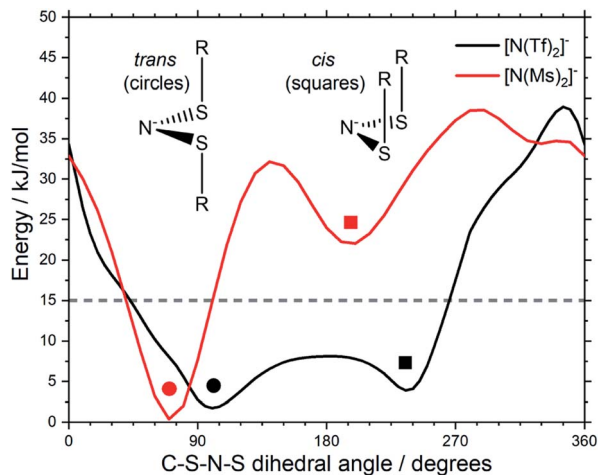
Fig. 12 Slices of the PES of [N(\text{Ms})_2]^- and [N(\text{Tf})_2]^- . One of the C–S–N–S dihedral angles is kept fixed ( 90^\circ for [N(\text{Tf})_2]^- , 80^\circ for [N(\text{Ms})_2]^- ).
