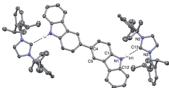
Fig. 3 ORTEP diagram (ellipsoids drawn at 50% probability) of BC·2IPr . Non-hydrogen bonding hydrogens and co-crystallized THF are omitted for clarity. Average select bond lengths (Å) and angles ( ^\circ ): \text{H1}\cdots\text{C13} , 2.10; \text{N1}\cdots\text{C13} , 2.96; \text{N2-C12-N3} , 102.2^\circ ; \text{N2-N3-C12-C1} , 13.5^\circ .
