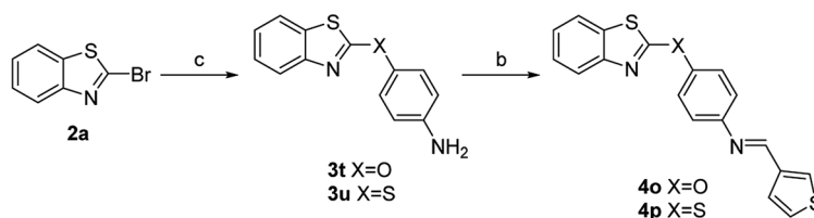
Scheme 2 Reagents and conditions. (a) 4-Aminophenylboronic acid pinacol ester, Pd(dppf)Cl 2 ·CH 2 Cl 2 , K 2 CO 3 , DMF, 70 °C, 16 h. (b) Thiophene-3-carbaldehyde, AcOH, MeOH, reflux, 2 h. (c) For 4o : 4-aminophenol, t -BuONa, K 2 CO 3 , DMF, room temperature, 5 h; for 4p : 4-amino-benzenethiol, K 2 CO 3 , MeCN, reflux, 3 h.
