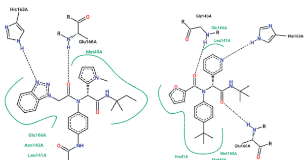
Fig. 8 The 2-D interaction profiles of the HTS hit compounds 49 (ML300; 4m5d.pdb) and 48 (ML188; 3v3m.pdb) in the active site residue of SARS-CoV-1 3CLpro; hydrogen bonds are shown with broken lines, and hydrophobic interactions are shown in green. The picture was prepared using the “poseview” tool.
