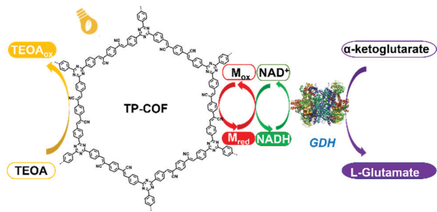
Fig. 10 Schematic illustration of the artificial photosystem I using TP-COF. Reproduced from ref. 117a with permission from Wiley-VCH Verlag GmbH & Co. KGaA, Copyright 2019.
