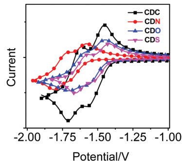
Fig. 7 Cyclic voltammogram of CDC, CDN, CDO and CDS, c = 1.0 \times 10^{-3} M. The deaerated acetonitrile solution contained the compounds, 0.10 M \text{Bu}_4\text{NPF}_6 as supporting electrolyte, \text{Ag}/\text{AgNO}_3 as a reference electrode, scan rates: 100 \text{ mV s}^{-1} . For all compounds, ferrocene (Fc) ( c = 1.0 \times 10^{-3} M) was used as an internal reference, 20^\circ\text{C} .
