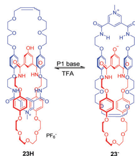
Fig. 23 pH-Switchable [2]catenane 23H driven by anion recognition.
