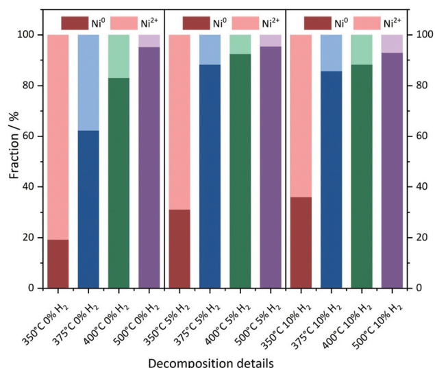
Fig. 5 Linear combination fitting of the XANES spectra. Ni foil and the Ni(BDC)(PNO) precursor were used as the \text{Ni}^0 and \text{Ni}^{2+} references, respectively.
