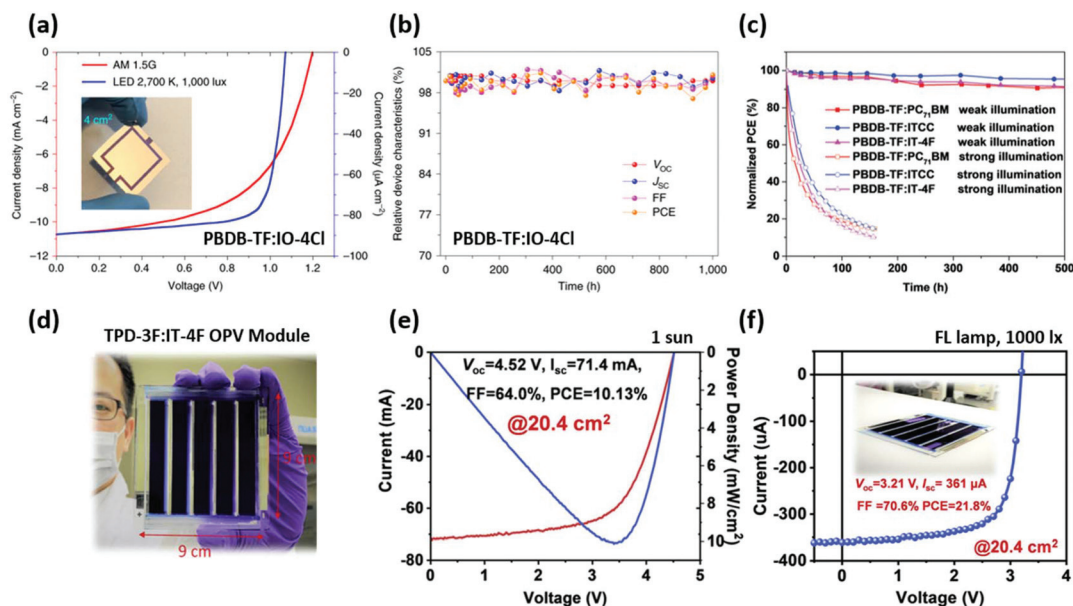
Fig. 8 Stable large-area indoor OPVs. (a) J–V characteristics of PBDB-TF:IO-4Cl devices (device area = 4 cm 2 ) under 1 sun and LED illumination. (b) Stability results of photovoltaic parameters versus time. Reproduced from ref. 32 with permission from Springer Nature. (c) Device stability of PBDB-TF blends with PC 71 BM, ITCC and IT-4F under weak and strong illumination. Reproduced from ref. 63 with permission from WILEY-VCH. Indoor OPV modules. (d) Photograph of OPV modules. (e and f) J–V characteristics of TPD-3F:IT-4F-based OPV modules under AM 1.5G and FL lamp (1000 lx) illumination, respectively. Reproduced from ref. 64 with permission from Elsevier.
