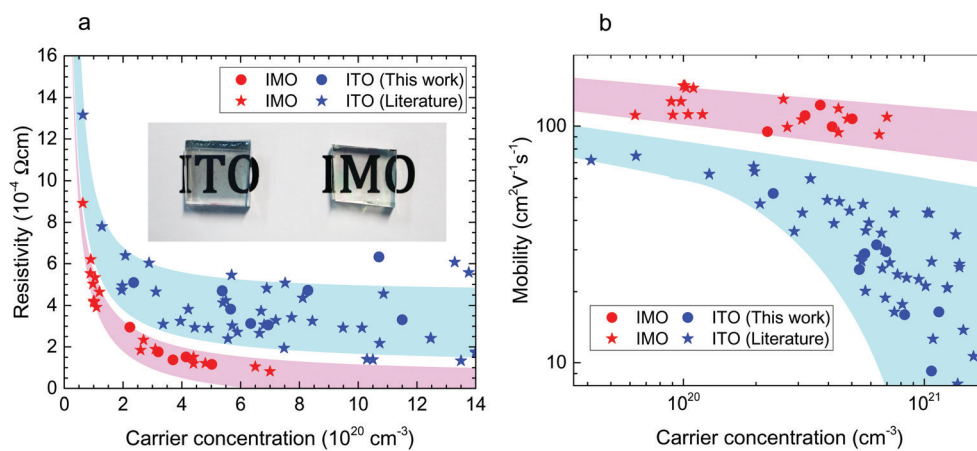
Fig. 2 Transport properties. (a) Resistivity versus free carrier concentration for polycrystalline ITO and IMO films. Inset shows a photograph of ITO and IMO films. (b) Hall mobility versus free carrier concentration. Data from this work are circles. Data plotted as stars are taken from the literature for IMO 11–16 and ITO 12,17–22 films. In this carrier concentration regime, the electron mobility is limited by ionized impurity scattering.
