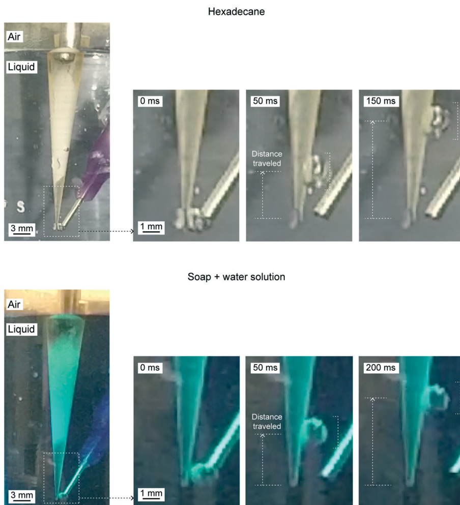
Fig. 24 Optical images of underwater air bubbles traveling on cones under various liquids (adapted from ref. 19).
