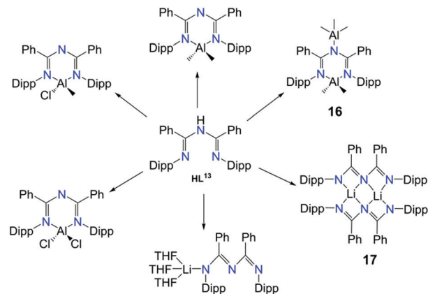
Scheme 10 The synthesis of mononuclear and dinuclear complexes of Al^{III} and Li^I with HL^{13} . 47
