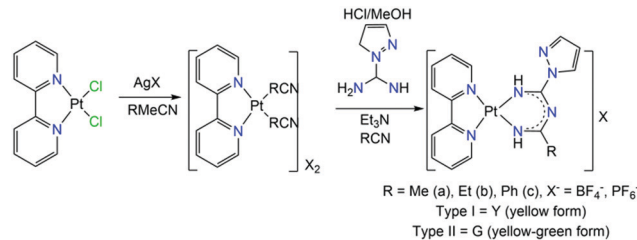
Scheme 17 Synthesis of [Pt II (bpy)(L 25R )]X ( 39R ) (where bpy = 2,2'-bipyridine, R = Me (a), Et (b) or Ph (c) and X = BF 4 - , PF 6 - ). 57
