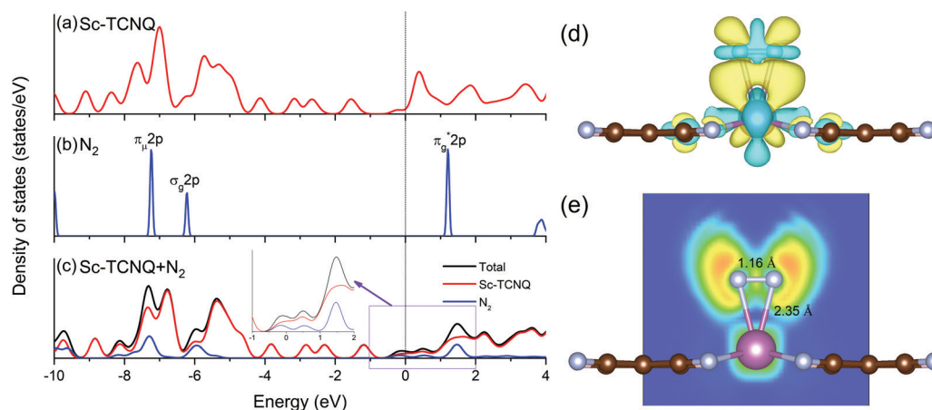
Fig. 4 Density of states of (a) pristine Sc-TCNQ, (b) N_2 molecule in the gas phase, and (c) Sc-TCNQ with one adsorbed N_2 molecule. Fermi level is set to zero and denoted in the black line. Inset in (c) shows the zoomed DOS near the Fermi level. (d) Charge density difference distribution (charge accumulation and depletion are shown in yellow and light blue, respectively) of N_2 adsorption with the side-on configuration, and (e) corresponding ELF map with bond lengths of Sc–N and N–N marked in the figure.
