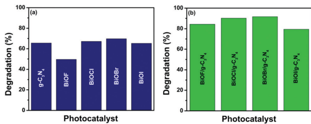
Fig. 9 Photocatalytic activity plots presenting the percentage of degradation of CR dye under sunlight irradiation for a stipulated time of 90 min using (a) bare BiOX and g-C 3 N 4 as catalysts and (b) different BiOX/g-C 3 N 4 composites as catalysts.
