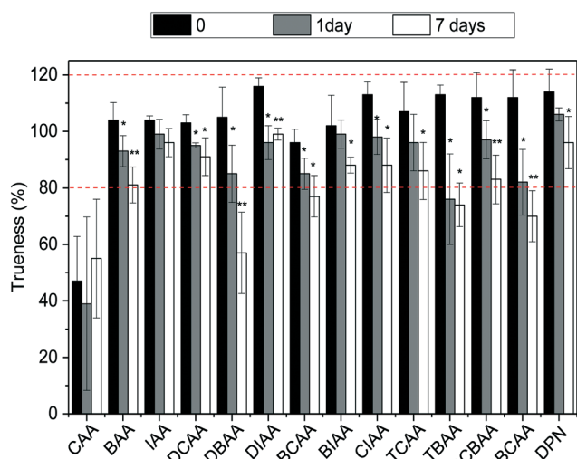
Fig. 3 Trueness values of HAAs and dalapon in tap water fortified at a concentration of 5 \mu\text{g L}^{-1} and stored at -20 \text{ }^\circ\text{C} for 7 days. Error bars indicate RSD values of n = 3 measurements.
