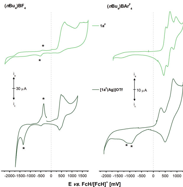
Fig. 9 Cyclic voltammograms of 1 mmol L -1 \mathbf{1a}^{\text{F}} (light green) and [\mathbf{1a}^{\text{F}}(\text{Ag})\text{OTf}] (dark green) in 0.1 mol L -1 supporting electrolyte solutions ( (n\text{Bu}_4\text{N})\text{BF}_4 (left) and (n\text{Bu}_4\text{N})\text{BARF}_4 (right) in \text{CH}_2\text{Cl}_2 ). Traces have been recorded at 100 mV s -1 (working electrode: glassy carbon, counter electrode: Pt wire) at room temperature. The second of three cycles are shown and asterisks (*) mark oxidation/reduction events which depend on prior oxidation in the first cycle ( cf. Fig. S66 and S67†).
