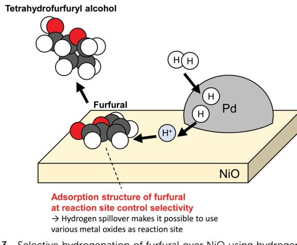
Fig. 3 Selective hydrogenation of furfural over \text{NiO} using hydrogen spillover from Pd.
