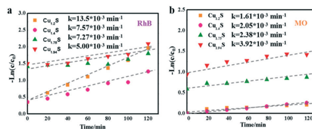
Fig. 7 Kinetic curves of the Cu 2-x S NCs for RhB (a) and MO (b) photodegradation under UV irradiation.
