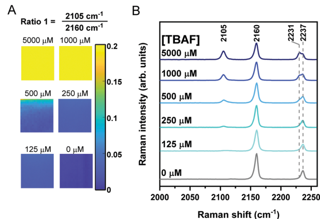
Fig. 4 Paper-based detection of fluoride using Raman sensor 1 . (A) Filter paper was pre-treated with sensor 1 (100 mM in THF, 10 \mu\text{L} ) before air-drying and subsequent direct addition of TBAF in THF (300 \mu\text{L} ) at the indicated concentrations. Raman maps were acquired across 20\ \mu\text{m} \times 20\ \mu\text{m} (1 \mu\text{m} pixel size; 400 spectra) using 785 nm laser excitation with a 20\times objective lens ( \sim 180 mW) for 0.5 s. The maps represent the ratio 2105\text{ cm}^{-1}/2160\text{ cm}^{-1} . For the blank sample, 10 mM TBACl replaced TBAF. (B) Average Raman spectra from maps presented in A. Peak annotations are in \text{cm}^{-1} .
