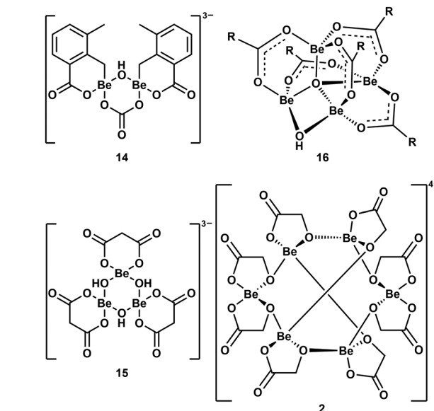
Fig. 8 Multinuclear beryllium compounds with bio-relevant ligands, which all contain six- or eight-membered beryllium heterocycles (R = 2-F-C 6 H 4 ). 39,41,57,58
