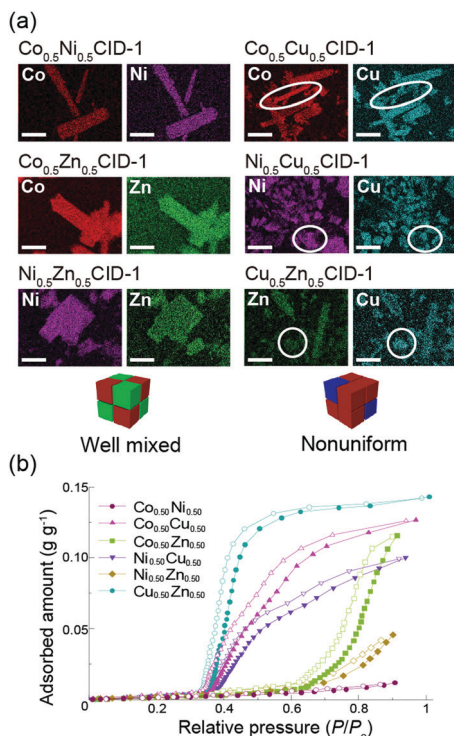
Fig. 4 (a) SEM-EDX maps for M_{1.5}M_{2.5}CID-1 . White circles indicate nonuniform areas. Scale bars: 30 \mu\text{m} . (b) Water-sorption isotherms of M_{1.5}M_{2.5}CID-1 at 298 K. Filled and open symbols correspond to adsorption and desorption, respectively.
