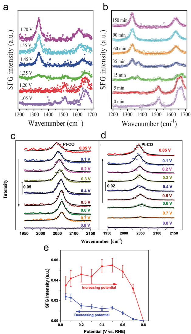
Fig. 8 Operando SFG spectra of HMF oxidation on Ni 3 N catalyst surfaces after 90 minutes at select potentials (referenced vs. RHE) (a) or as a function of time at 1.45 V (b). CO was detected on polycrystalline Pt surfaces at low potentials and was more prevalent in the forward scan (c) than in the reverse scan (d). The intensities of the CO band as a function of potential are plotted in (e). Reprinted with permission from ref. 44 (N. Zhang, Y. Zou, L. Tao, W. Chen, L. Zhou, Z. Liu, B. Zhou, G. Huang, H. Lin and S. Wang, Angew. Chem., Int. Ed. , 2019, 58 , 15895–15903) and ref. 45 (Y. Liu, W. Yu, D. Raciti, D. H. Gracias and C. Wang, J. Phys. Chem. C , 2019, 123 , 426–432). Copyright John Wiley and Sons 2020 and American Chemical Society 2019.
