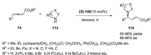
Scheme 54 Phosphine-catalysed \gamma -addition of substituted pyrazoles, imidazoles and oxazolones.
