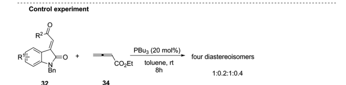
Scheme 10 Phosphine-catalysed highly diastereoselective (3+2) annulations of isatin derived electron-deficient alkenes.
