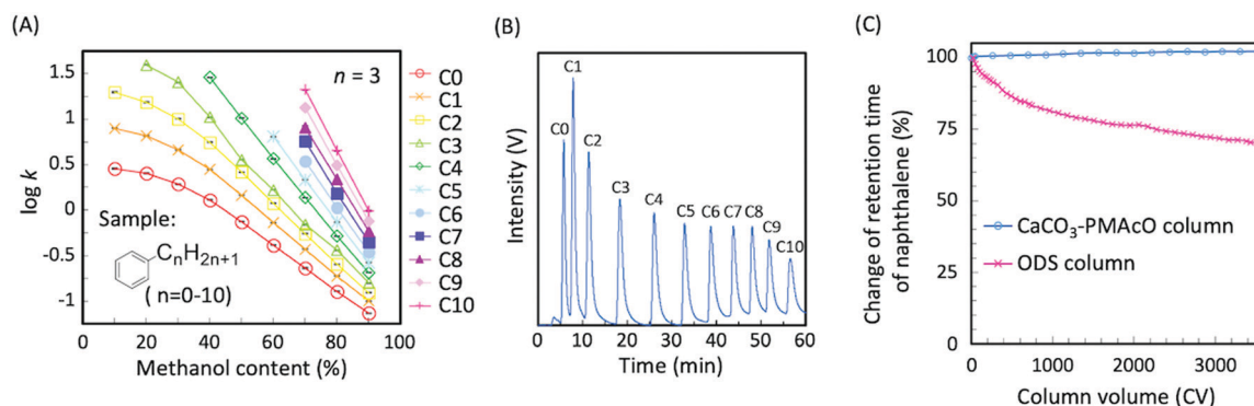
Fig. 4 (A) Retention factors of C0–10 alkylbenzenes obtained with a \text{CaCO}_3 -PMAcO packed column. Each sample was eluted at each mixing ratio of the methanol/water mobile phase ranging from 10/90 (v/v) to 90/10 (v/v); error bars represent mean values \pm 1\sigma ( n = 3 ); flow rate of mobile phase 0.3 \text{mL min}^{-1} . (B) Chromatogram showing the separation of a mixture of C0–10 alkylbenzenes by the \text{CaCO}_3 -PMAcO column. Gradient elution was applied at a flow rate of 0.1 \text{mL min}^{-1} starting with methanol/water (50/50, v/v) for 4 min, followed by the gradient program up to 80/20 (v/v) over 36 min and finally elution with 80/20 (v/v) for 20 min. (C) Relative change of the retention time of naphthalene upon continuous running of alkaline mobile phase (50/50, v/v methanol/pH 10.8 \text{Na}_2\text{B}_4\text{O}_7 buffer) in the case of \text{CaCO}_3 -PMAcO and ODS columns; flow rate of mobile phase 0.3 \text{mL min}^{-1} .
