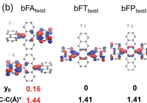
Fig. 5 (a) Energy diagram of \text{bFA} with rotation of the fluorene moiety; (b) HOMOs of the fluorene twisted structure of \text{bFA} ( \text{bFA}_{\text{twist}} ), \text{bFT} ( \text{bFT}_{\text{twist}} ), and \text{bFP} ( \text{bFP}_{\text{twist}} ), with the y_0 value and bond length (*) of the C–C bond between fluorene and acenes.
