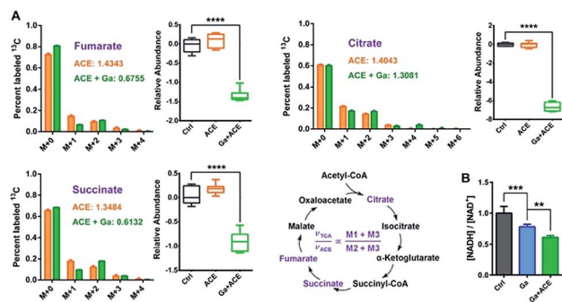
Fig. 5 Combined Ga(III) and acetate treatment leads to reduced TCA cycle flow. (A) Mass isotopomer distributions of 13 C 2 -labelled acetate detected in the TCA cycle and the relative abundances of cycle metabolites. (B) Ratios of bacterial cellular NADH and NAD + levels after treatment with Ga(III) and acetate. Data are presented as mean ± SEM from biological replicates. The asterisks indicate significant difference from the Ctrl or Ga(III) treatment group (**, 0.001 < p < 0.01 and ***, p < 0.001).
