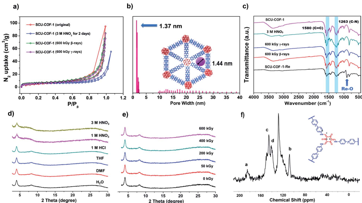
Fig. 2 (a) \text{N}_2 sorption isotherms of SCU-COF-1 after different treatments with 3 M \text{HNO}_3 , 600 kGy \beta -rays, and 600 kGy \gamma -rays at 77 K. (b) Pore size distribution of SCU-COF-1 calculated by NLDFT modelling based on \text{N}_2 adsorption data. (c) IR spectra of SCU-COF-1 and SCU-COF-1 after treatment with 3 M \text{HNO}_3 , 600 kGy \gamma -irradiation, 600 kGy \beta -irradiation, and stock solution containing \text{ReO}_4^- . (d) PXRD patterns of SCU-COF-1 after treatments in various solvents and acids for 48 h. (e) PXRD patterns of SCU-COF-1 after being irradiated with various doses of \beta -irradiation (50 kGy, 200 kGy, 400 kGy, 600 kGy). (f) ^{13}\text{C} solid NMR spectrum of SCU-COF-1.
