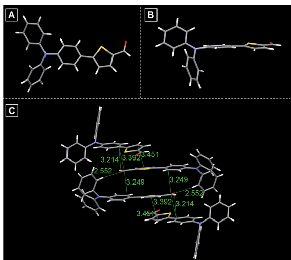
Fig. 2 (A) Single crystal structure of TTB. (B) Side view of the crystal structure of TTB. (C) Various inter- and intramolecular interactions in crystals of TTB.
