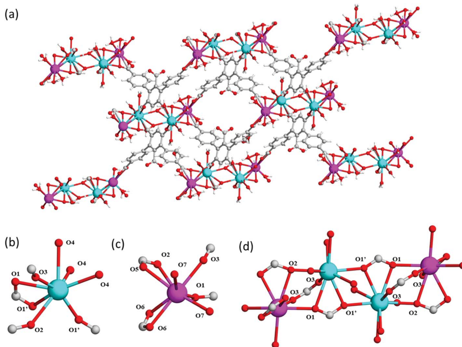
Fig. 4 View of (a) the crystal structure of MFM-512 along the a -axis; (b) type I) and (c) type II) Ba(II) nodes in MFM-512 showing distorted octahedral and trigonal prismatic square face monocationic coordination, respectively. H-atoms are omitted for clarity; (d) View of the tetranuclear Ba(II) cluster in MFM-512. Carbon, grey; oxygen, red; hydrogen, white; barium, magenta (type I) and cyan (type II).
