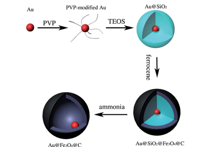
Fig. 8 Schematic of the preparation procedure of yolk-type Au@Fe 3 O 4 @C. 80
