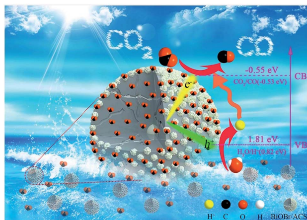
Scheme 2 Possible mechanism of the photocatalytic \text{CO}_2 reduction to CO over BiOBr/ACSS.
