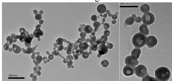
Fig. 3 Top: Emission spectra of ppy-Pt-3-Cl-(S,S)Cy in THF and THF/water ( 2.0 \times 10^{-5} mol \text{dm}^{-3} ). Inset: Their photographs under room light and 360 nm UV light. Bottom: Transmission electron microscopy of ppy-Pt-3-Cl-(S,S)Cy (THF/water, 96% water) on carbon-coated copper grids after solvent evaporation.
