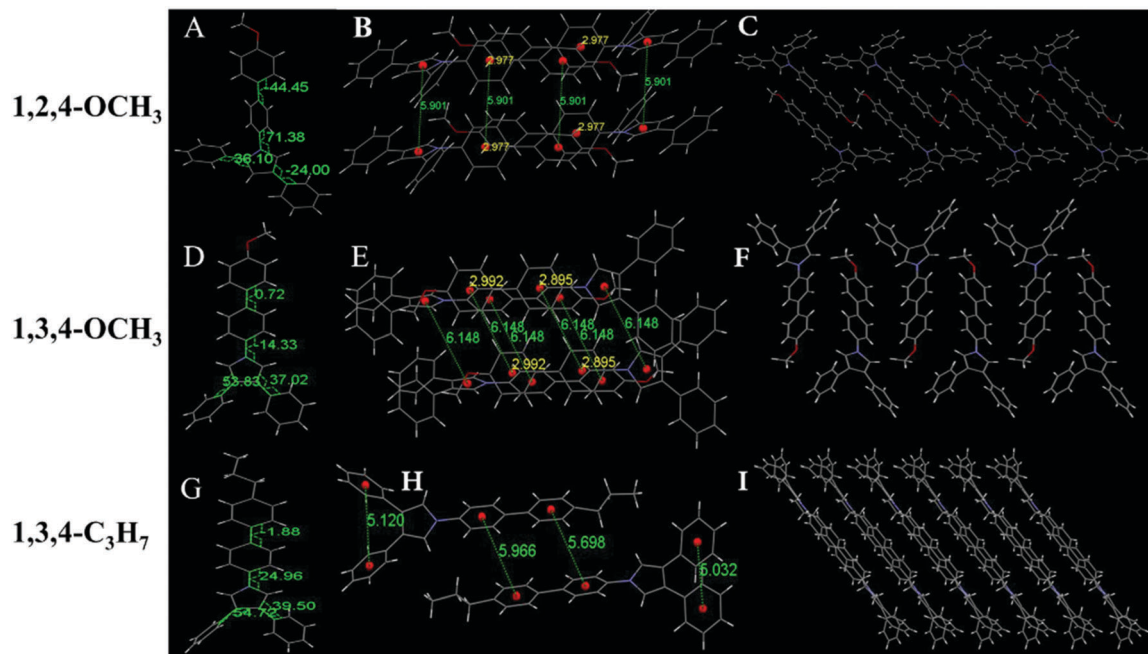
Fig. 3 (A) Molecule structure, (B) interaction distance of the \pi\cdots\pi and C–H \cdots\pi interactions and (C) stacking image along the b -axis of 1,2,4-OCH 3 . (D) Molecular structure, (E) interaction distance of the \pi\cdots\pi and C–H \cdots\pi interactions and (F) stacking image along the b -axis of 1,3,4-OCH 3 . (G) Molecular structure, (H) interaction distance of the \pi\cdots\pi and C–H \cdots\pi interactions and (I) stacking image along the b -axis of 1,3,4-C 3 H 7 . Gray color corresponds to carbon, white to hydrogen, red to oxygen and blue to nitrogen.
