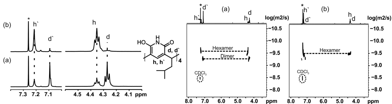
Fig. 2 Left: 1 H NMR of 1 (20 mM in CDCl 3 ) (a) measured within 2 hours after sample preparation and (b) same sample after 7 days from sample preparation. Right: DOSY NMR of the same sample (a) measured within 2 hours from sample preparation and (b) after 7 days from sample preparation. Signals d and d' correspond to the dimeric assembly and signals h and h' to the hexameric assembly.
