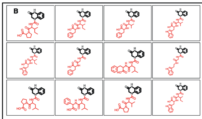
Fig. 4 (A) Top: feature frequency plot for GNPS Mass2Motif 60; middle: most enriched ClassyFire substituent terms in the same motif; bottom: MAGMa assigned the quinoxalino substructure in 22 of the 25 molecules associated to this motif. (B) Screenshot of the ms2lda.org web app with the MAGMa annotated quinoxalino substructure highlighted in 12 of the 22 molecules.
