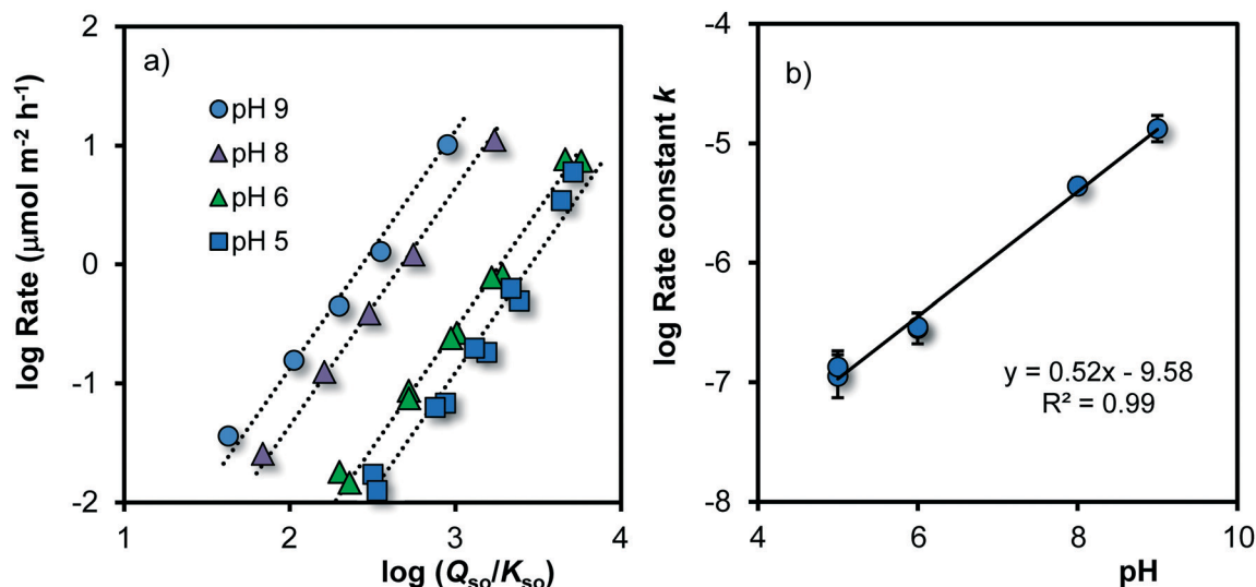
Fig. 5 a. Logarithm of the rate of growth R ( \mu\text{mol m}^{-2} \text{h}^{-1} ) as a function of the logarithm of the super saturation of the solution ( Q_{so}/K_{so} ) for Fh in 0.2 M \text{NaNO}_3 buffered with 19 mM MES and 19 mM MOPS at the given pH values ( T = 20^\circ \text{C} ). The slopes of the calculated lines ( s ) have been set to s = 2 . The intercept at \log(Q_{so}/K_{so}) = 0 equals the logarithm of the rate constant ( \log k ), which is plotted in Fig. 5b against the pH, revealing the pH dependency of \log k (eqn (8)) with k in \mu\text{mol m}^{-2} \text{h}^{-1} .
