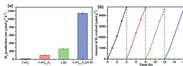
Fig. 6 (a) Comparison of the \text{H}_2 evolution rate of \text{CeO}_2 , \text{CeO}_{2-x}\text{S}_x , CdS and \text{CeO}_{2-x}\text{S}_x@\text{CdS} photocatalysts and (b) stability test of \text{H}_2 evolution for \text{CeO}_{2-x}\text{S}_x@\text{CdS} under visible-light irradiation ( \lambda > 420 \text{ nm} ).
