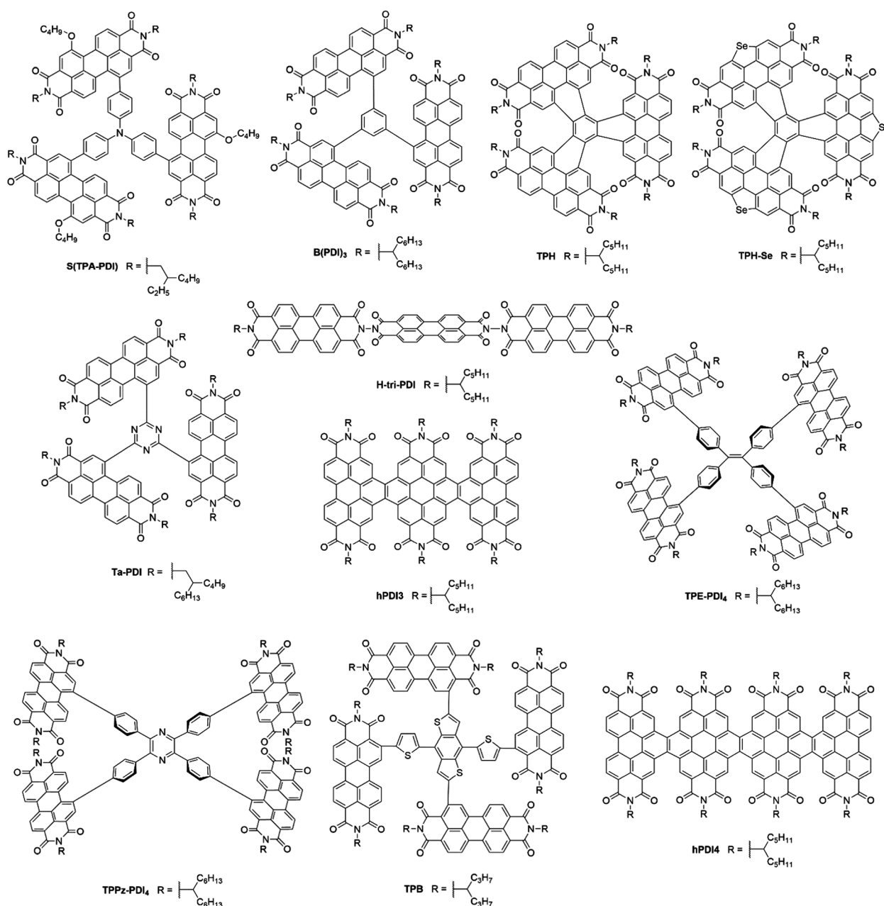
Fig. 10 Trimeric and tetrameric PDI based small molecule acceptors.
