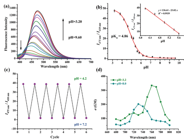
Fig. 1 (a) Emission spectra of Lyso-MPCB (10 \mu\text{M} ) in B–R buffer solution with different pH from 9.60 to 3.20 (with 30% DMSO, \lambda_{\text{ex}} = 370 nm). (b) Plot of the fluorescence intensity ratio ( I_{475\text{nm}}/I_{410\text{nm}} ) vs. pH. Inset: Linear relationship of pH-dependent fluorescence intensity ratio ( I_{475\text{nm}}/I_{410\text{nm}} ). R^2 = 0.9939 . (c) pH reversibility of Lyso-MPCB in B–R buffer solution (pH = 4.20 and 7.20). (d) Two-photon absorption cross-section of Lyso-MPCB with pH = 3.2 and 8.0, respectively. ( \lambda_{\text{ex}} = 680–800 nm).
