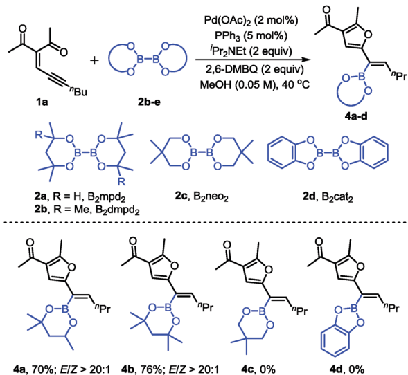
Scheme 3 Scope of the diboron compounds. Reaction conditions: 1a (0.2 mmol), 2b–e (0.4 mmol), \text{Pd(OAc)}_2 (2 mol%), \text{PPh}_3 (5 mol%), \text{{}^i\text{Pr}_2\text{NEt}} (0.4 mmol), and 2,6-DMBQ (0.4 mmol) in MeOH (4 mL) at 40 °C for 10 h. Isolated yields. The E/Z ratio was determined by ^1\text{H NMR} .
