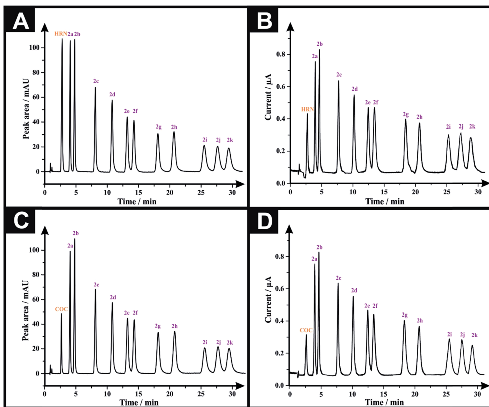
Fig. 2 (A) Representative HPLC-DAD chromatograms for a solution containing 50 μg mL -1 of each of HRN, fentanyl (2c) and fentanyl derivatives (2a, 2b, 2d–2k) using an Eclipse XDB-C8 column (150 × 4.6 mm, i.d. 5 μm); mobile phase: acetonitrile : 20 mM ammonium formate–100 mM potassium chloride buffer (pH 7.0) (30 : 70% v/v); flow rate 1.5 mL min -1 , detector wavelength (UV): 205 nm and column temperature: 25 °C. (B) Representative amperogram for a solution containing 50 μg mL -1 of each of HRN, fentanyl and its 10 derivatives obtained using HPLC-AD flow cell system. (C) HPLC-DAD chromatogram for a solution containing 50 μg mL -1 of each of COC, fentanyl and its 10 derivatives. (D) Representative amperogram for a solution containing 50 μg mL -1 of each of COC, fentanyl and its 10 derivatives obtained using HPLC-AD flow cell system.
