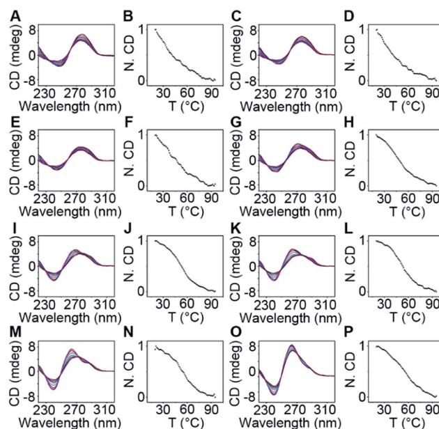
Fig. 5 CD spectra at 25, 35, 45, 55, 65, 75, 85, 95 and 99 ^{\circ} C (from top to bottom) at 264 nm, and normalized CD intensities (N. CD) as a function of temperature recorded at 264 nm with the temperature increased by 1.0 ^{\circ} C per 0.5 min of 20 \mu M (A and B) O1'-1G, (C and D) O1'-2G, (E and F) O1'-3G, (G and H) O1'-4G, (I and J) O1'-5G, (K and L) O1'-6G, (M and N) O1'-7G, and (O and P) O1'-8G. Data are normalized to the highest CD value of 264 nm.
