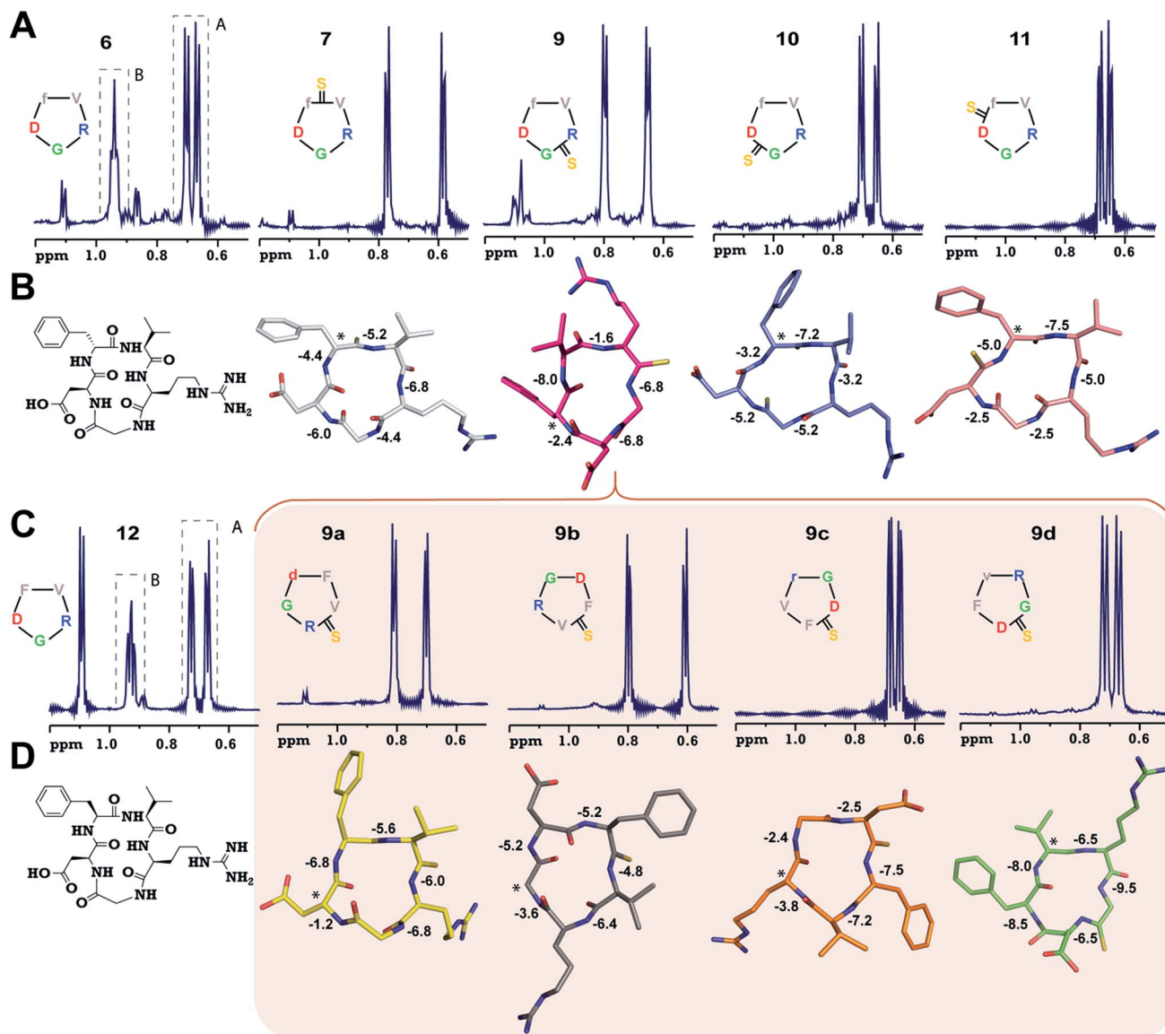
Fig. 2 (A) ^1\text{H} NMR spectra of cyclo(RGDfV) ( 6 ) and its thio-analogs 7–11 . The \gamma\text{-CH}_3 of Val in both the conformers (A and B) of 6 is shown. (B) The solution structures of 7–11 deduced from 2D ^1\text{H} NMR spectroscopy in aqueous conditions. (C) ^1\text{H} NMR spectra of cyclo(RGDfV) ( 12 ) showing two conformers. (D) Solution structures of spatial screen analogs of 9 ( 9a–9d ). The temperature coefficients of the amide protons (ppb \text{K}^{-1} ) are shown and the asterisk denotes the site of the D-amino acid (Gly in 9b ). Significant resonance overlap precluded the structure determination of 6 and 12 . The hydrogen atoms are omitted for the sake of clarity.
