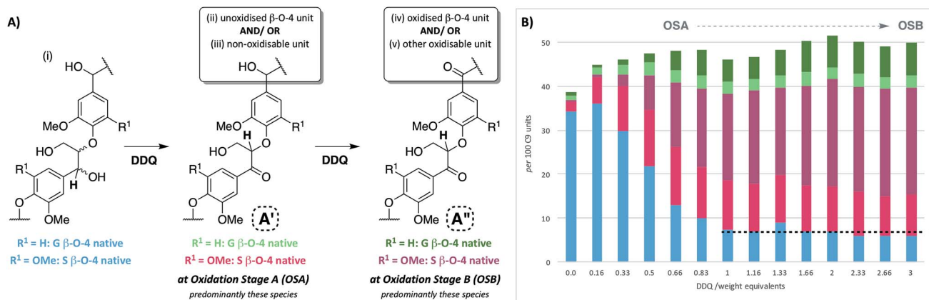
Fig. 3 Beech lignin DDQ oxidation study: (A) proposed reactivity of \beta -O-4 units within lignin including possible oxidized stages within lignin \alpha -ox of the \beta -O-4 unit. The chemical shifts of the highlighted H atoms are reliant on the substituents on the aromatic ring connected via the aryl-ether linkage (Fig. S1†); (B) graph displaying \beta -O-4 and \beta -O-4 \alpha -ox units per 100 C9 units against DDQ weight equivalents; highlighted H atoms (and their corresponding cross-peaks within 2D HSQC analysis) were used for semi-quantification of units within lignin. 38 Data repeated in triplicate, for standard error analysis, see Table S3.† All standard errors associated with values in this figure are <1.5%. *Dashed lines indicate a plateau where no more oxidation was notably occurring. No/very little signal corresponding to remaining \beta -O-4 native units were observed at this point in 2D HSQC NMR spectra, but background noise and/or new peaks may be overlapping with integral regions rendering these integrals not equal to zero.
