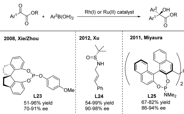
Scheme 17 Catalytic asymmetric 1,2-addition of arylboronic acids to \alpha -ketoesters.
