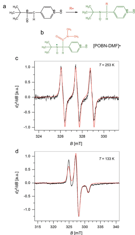
Fig. 6 (a) Scheme for the reaction of \alpha -4-pyridyl-1-oxide- N - tert -butylnitron (POBN) with free radicals to generate the corresponding spin-trapped nitroxide radical. (b) Chemical structure of a DMF radical trapped by POBN. (c) X-band EPR spectra obtained from spin-trap (POBN) experiments carried out on the supernatant from a GrF/DMF/POBN mixture ( T = 253 K) together with its EPR simulation (red-trace), and (d) corresponding spectrum obtained in a frozen matrix ( T = 133 K) compared with simulation (red-trace). Experimental parameters: 9.16–9.17 GHz frequency, 100 kHz modulation frequency, 30 ms time constant, 0.2 mT (c) or 0.8 mT (d) modulation width, 0.3 mW (d) or 4.0 mW (c) applied microwave power. Simulation parameters are given in the text.
