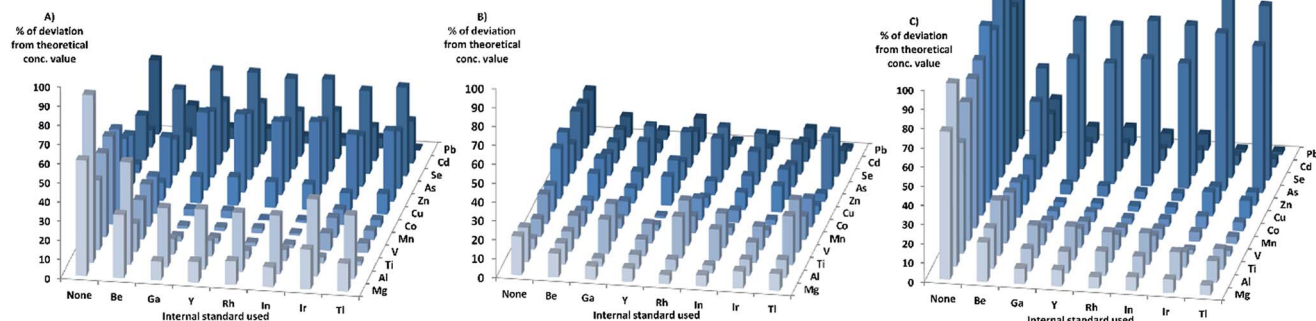
Fig. 2 Highest absolute deviation from theoretic concentration values for all matrix compositions in KED-mode, when using 1% HNO 3 -matrix for calibration. Scale restricted to a maximum of 100% deviation. (A) HNO 3 , (B) PBS, (C) Triton.
